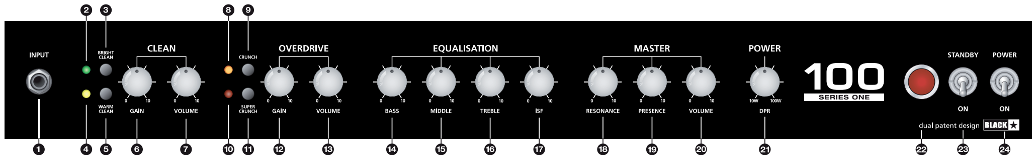
Front Panel
